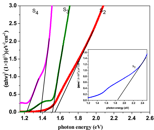
Fig. 4. Graph of (\alpha hv)^2 versus photon energy for all the samples.
