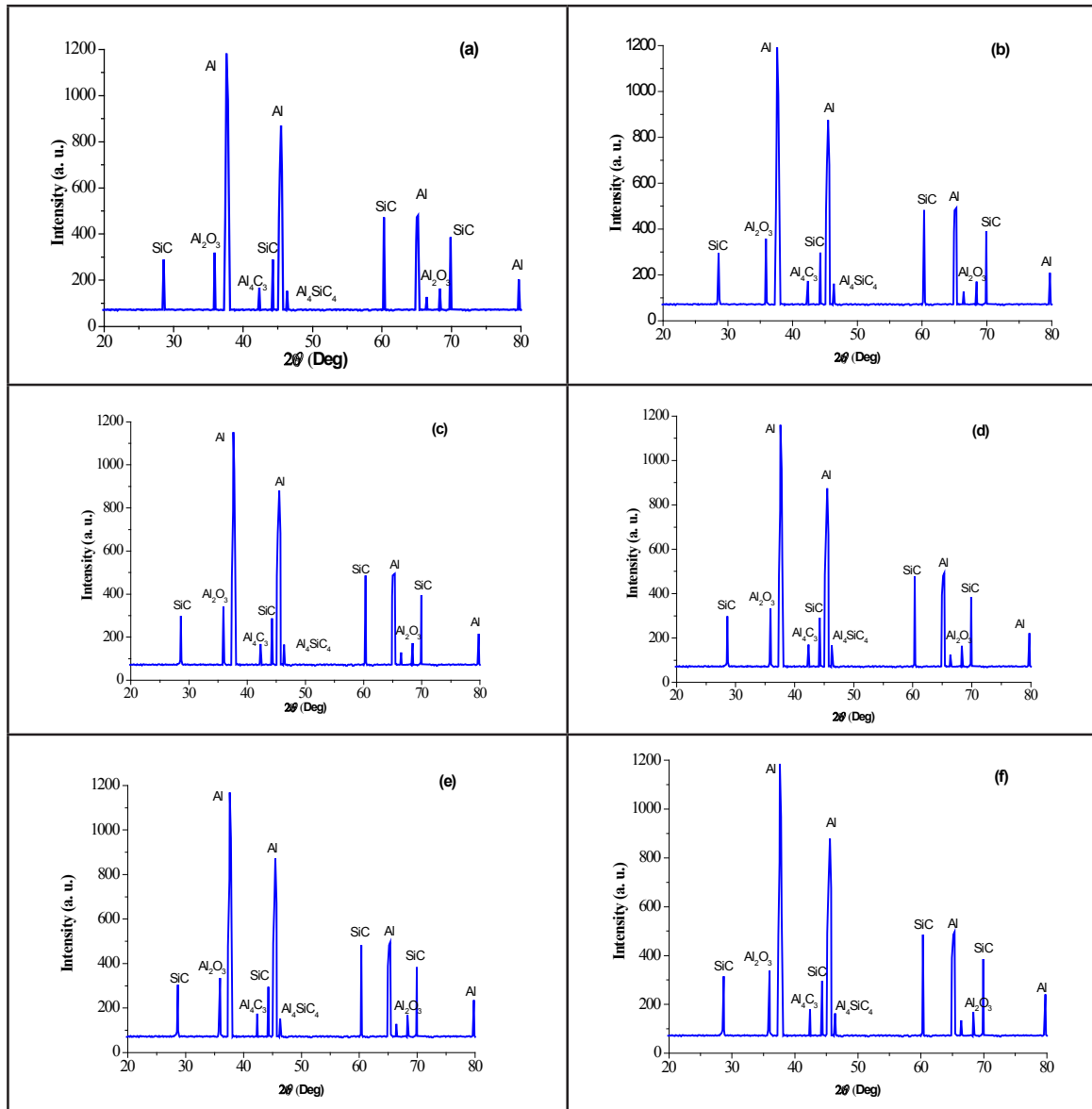
Fig. 5. XRD pattern for the samples (a) AA2024/0.5wt% \text{Al}_2\text{O}_3 /0.5wt%SiC, (b) AA2024/1wt% \text{Al}_2\text{O}_3 /1wt%SiC, (c) AA2024/2wt% \text{Al}_2\text{O}_3 /2wt%SiC, (d) AA2024/3wt% \text{Al}_2\text{O}_3 /3wt%SiC, (e) AA2024/4wt% \text{Al}_2\text{O}_3 /4wt%SiC, and (f) AA2024/5wt% \text{Al}_2\text{O}_3 /5wt%SiC.
