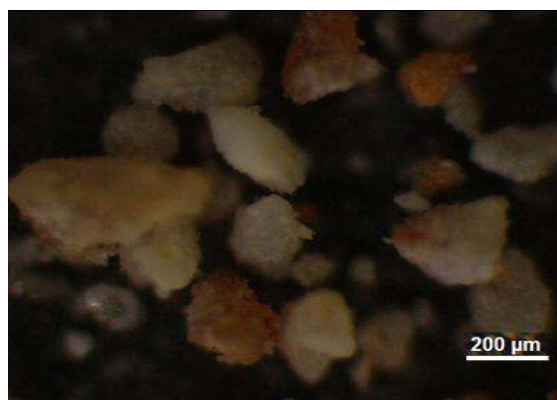
Fig.3. Optical microscopy image of the non-mechanically activated gold ore.
