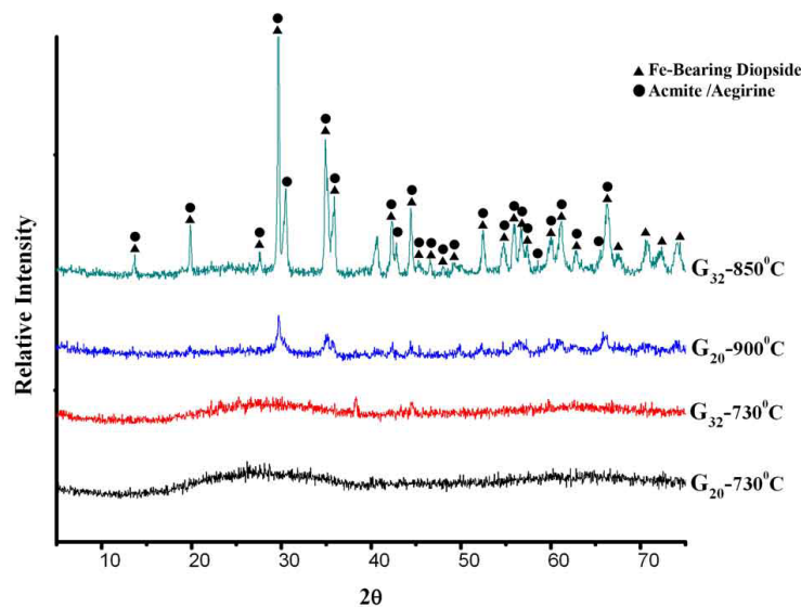
Fig. 3. XRD patterns of glasses G 20 and G 32 after heat treatment at 730°C and 900°C for 10 min.
