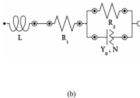
Fig. 4. a) Nyquist plots of contact paste at 800 °C and b) Corresponding equivalent circuit.
