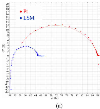
Fig. 4. a) Nyquist plots of contact paste at 800 °C and b) Corresponding equivalent circuit.
