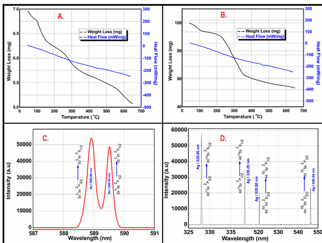
Fig. 6. DSC curves (blue lines) of NF (A) and NFC (B), respectively. TGA curves (black lines), NF in Figure (A) and NFC in Figure (B). Figures (C) and (D) show NFC LIBS analysis spectra. The spectroscopic signature of silver (Ag) and sodium (Na) observed in NFC emission spectrum.
