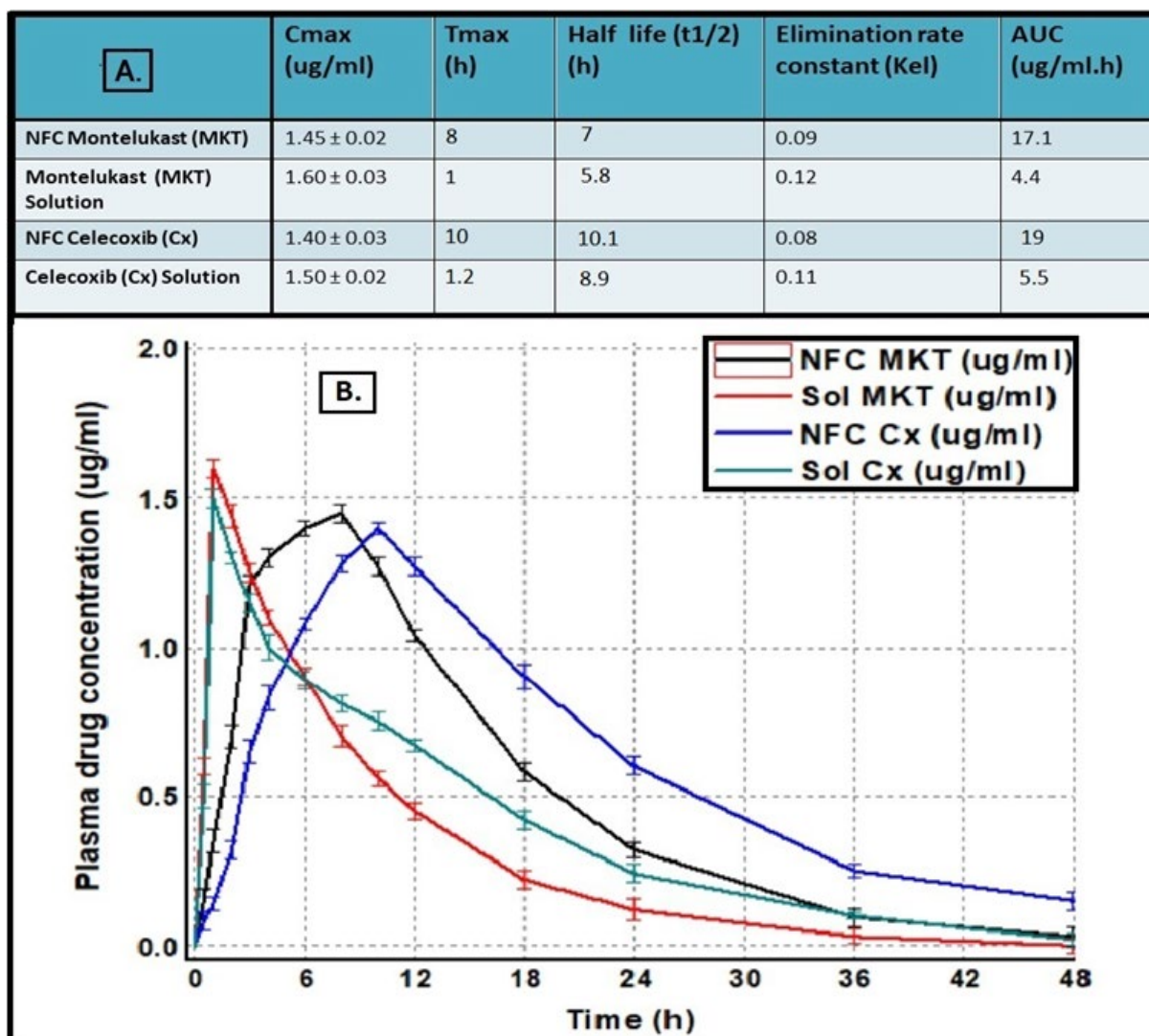
Fig. 17. A) In-vivo pharmacokinetic parameters of NFC, CX solution and MKT solution B) In-vivo plasma drug concentrations at specified time intervals after single oral dose administration.
