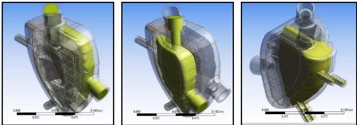
Fig. 2. The 3D models for the designed soft artificial heart; (a) the right and; (b) the left ventricles; (c) the air pressure and drag zones
