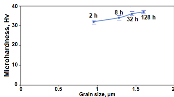
Fig. 13. Relationship between the hardness and the grain size of Zn-22Al alloy after post-ECAP aging at 100°C.
