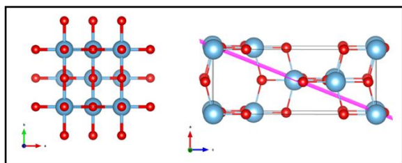
Fig. 4. Crystal structure of Anatase TiO_2 and its (101) plane
