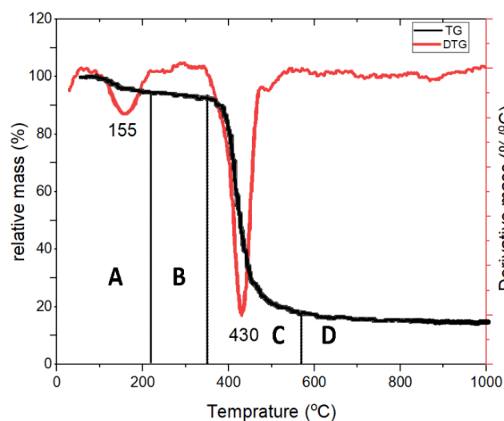
Fig. 11. The TG/DTG analysis of the resin sample
