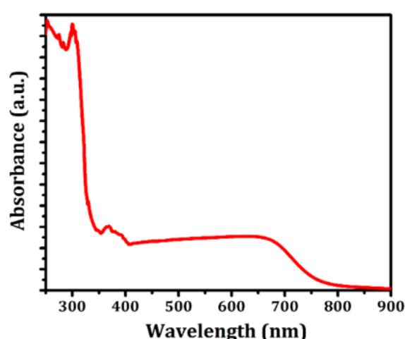
Fig. 4. UV-visible absorption spectra.
