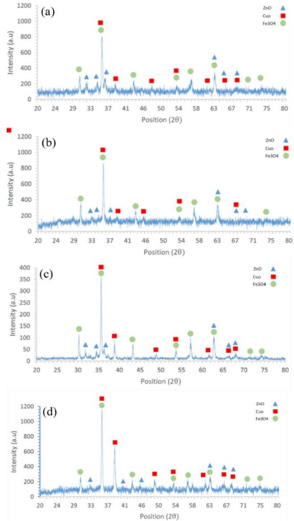
Fig. 2. XRD patterns of synthesized \text{Fe}_3\text{O}_4/\text{ZnO}/\text{CuO} nanocomposite: a) \text{Fe}_3\text{O}_4/\text{ZnO}/\text{CuO} (1:1:0.3), b) \text{Fe}_3\text{O}_4/\text{ZnO}/\text{CuO} (1:1:0.5), c) \text{Fe}_3\text{O}_4/\text{ZnO}/\text{CuO} (1:1:1) and d) \text{Fe}_3\text{O}_4/\text{ZnO}/\text{CuO} (1:1:3)
