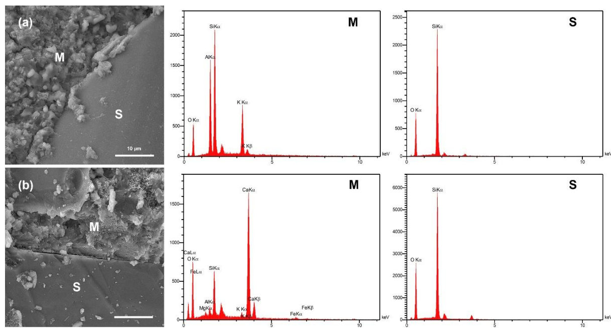
Fig. 9. Microstructure of a) geopolymer concrete (GS20) and b) Portland cement concrete (PS20) with EDX patterns of matrix (M) and quartz sand (S)
