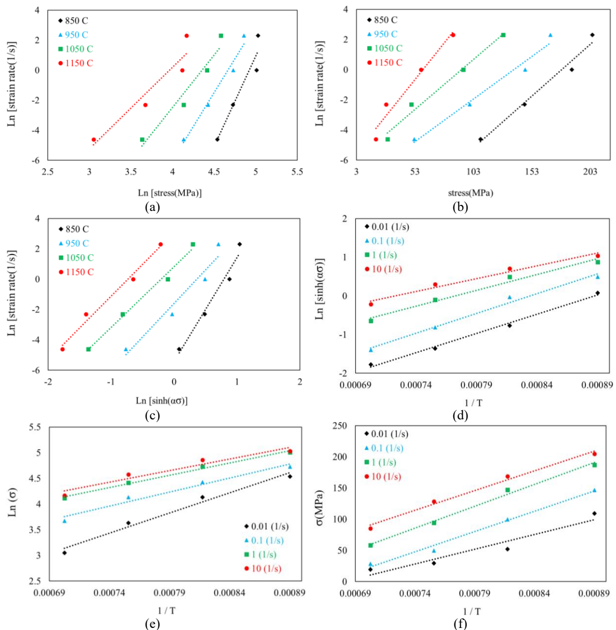
Fig. 6. Arrhenius-type plots for the FBN sample: natural logarithm of a) power, b) exponential, and c) hyperbolic sine functions vs. strain rate, and d-f) their relations with inverse absolute temperature at different conditions
