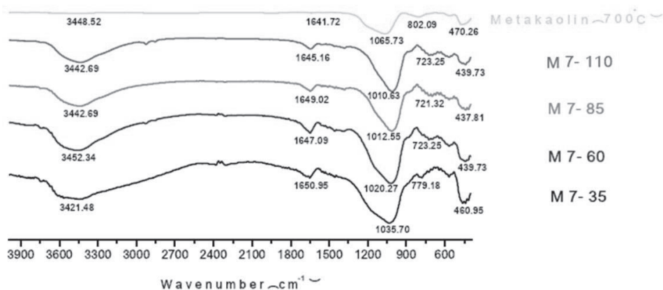
Fig. 5. FTIR spectra of the metakaolin calcined at 700 °C and geopolymer cements after 28 days curing with different molar ratio of Na 2 O/SiO 2 .
