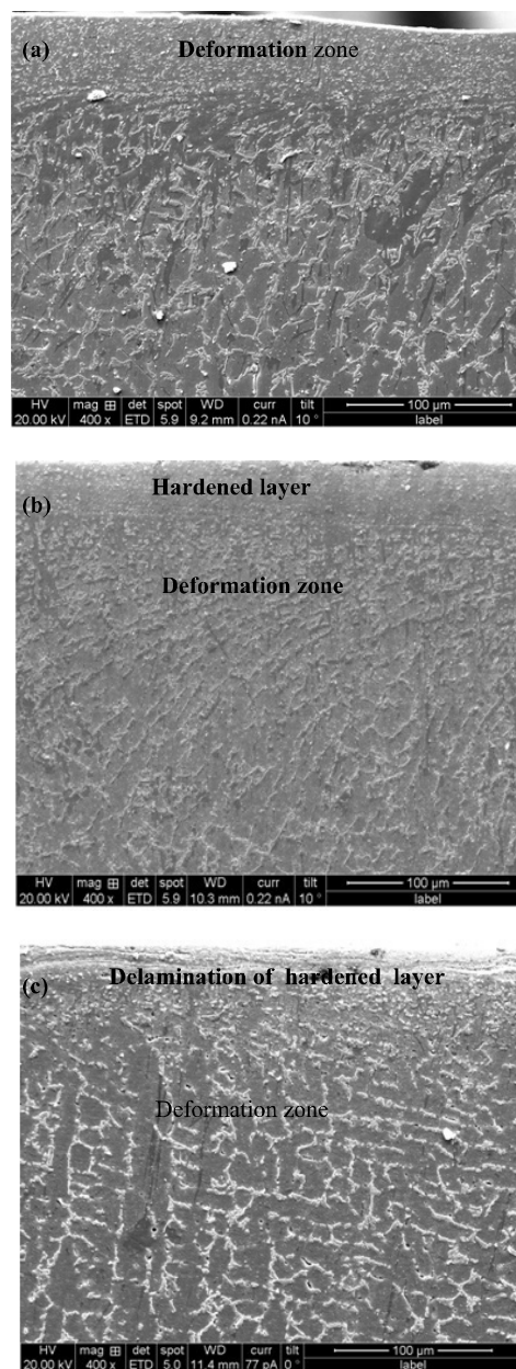
Fig. 9. SEM showing subsurface features in base alloy (a). formation of deformation zone (b). formation of hardened layer (c). delamination of hardened layer
