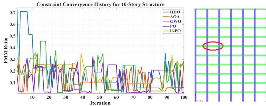
Figure 15: PMM interaction ratio convergence history for a representative beam in the ten-story steel frame structure.
