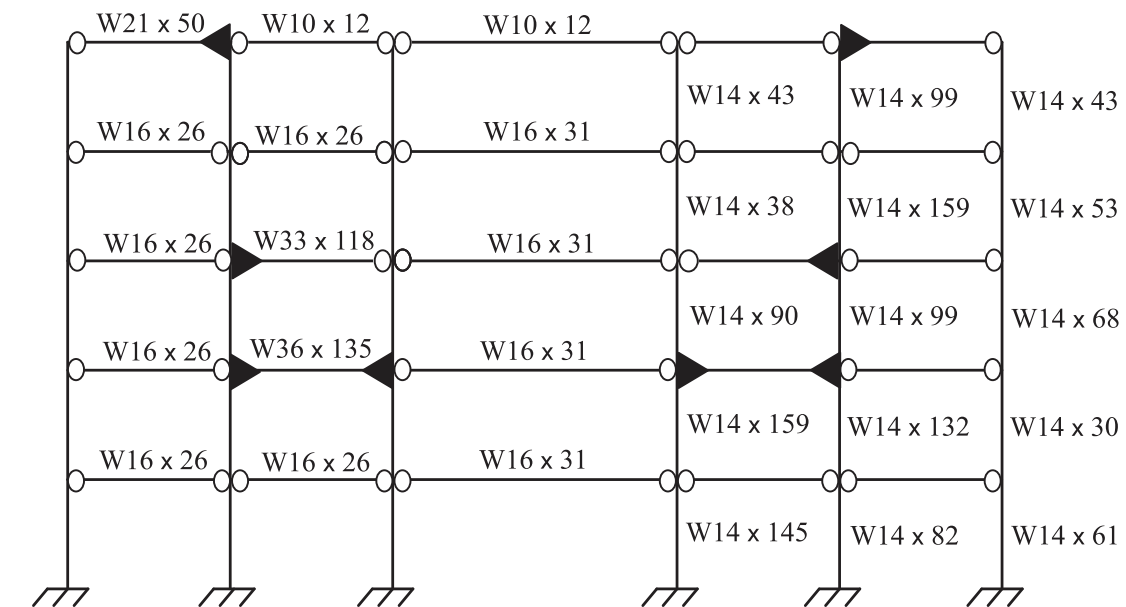
Figure 20. Best 5 \times 5 designs from binary genetic algorithm with variable connection topology in two pools by including constraints
