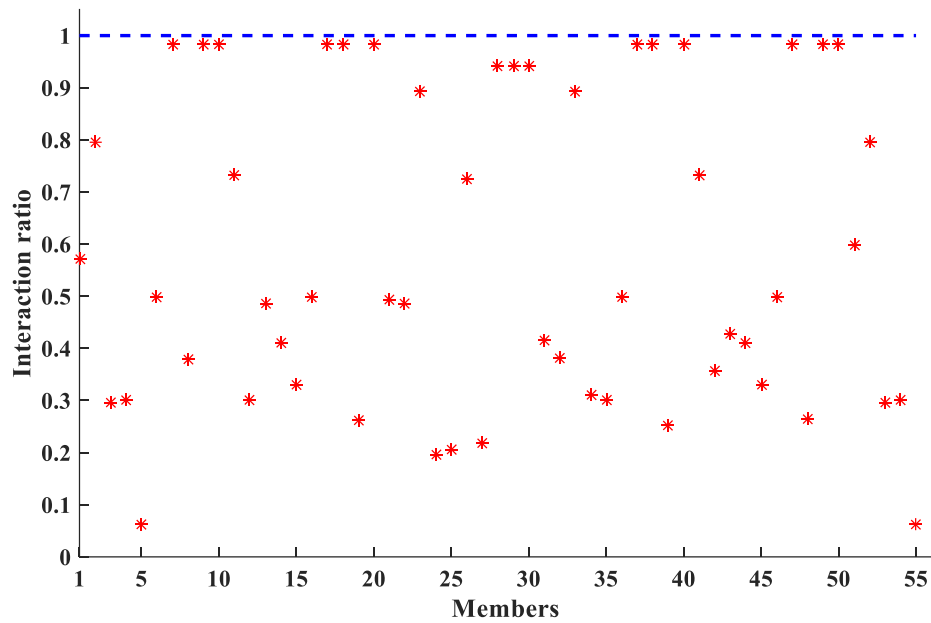
Figure 19. Members interaction ratio of 5 \times 5 frame with variable connections for mode 3
